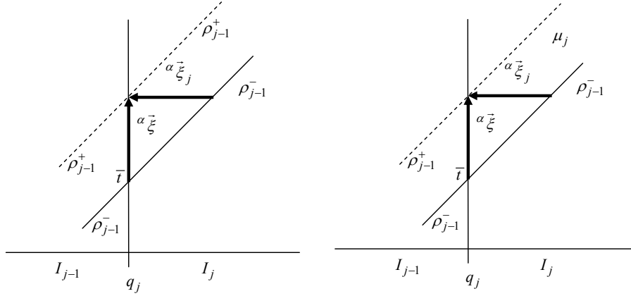
FIG. 6.1. \rho_{j-1}^+ < \rho_{j-1}^- (left) and \rho_{j-1}^+ > \mu_j (right): the non shifted wave is represented by a continuous line, while the shifted ones by a dashed line.
